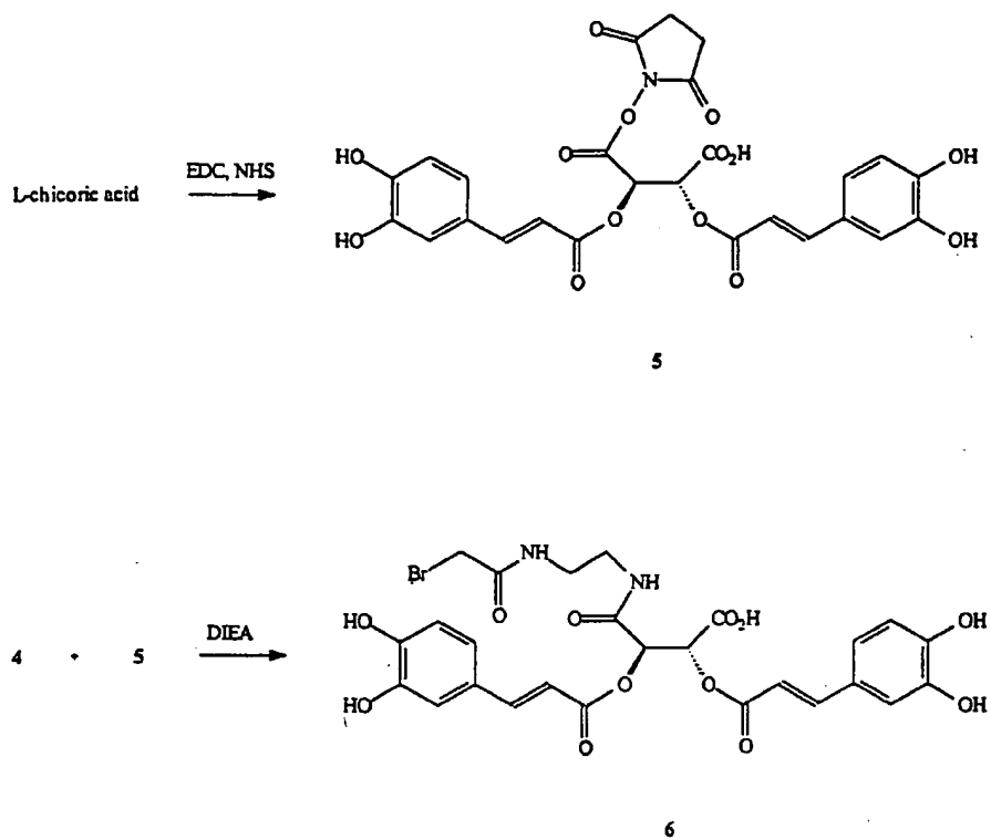
Scheme 3 Synthesis of bromoacetylated derivative of L-chicoric acid
